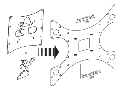
Piastra VESA 10x10 cm VESA plate 10x10 cm
